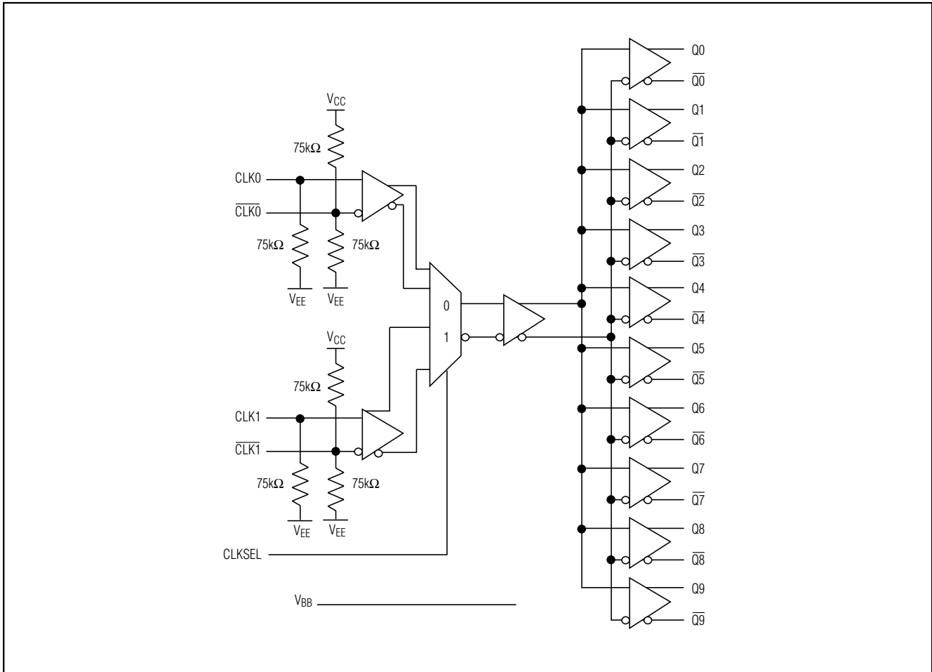
Functional Diagram
