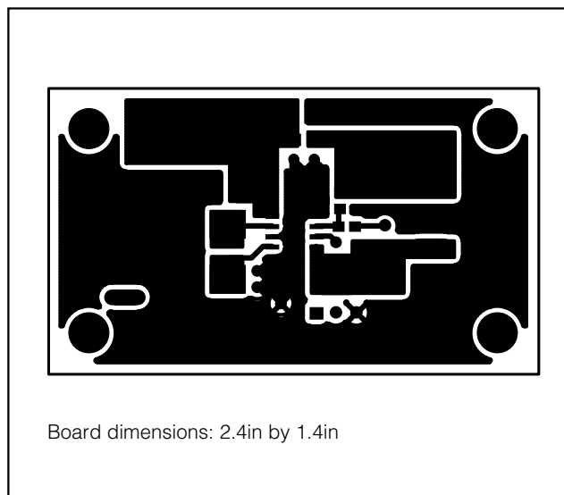
Figure 3. MAX889S EV Kit PC Board Layout—Component Side
