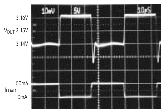
LOAD-TRANSIENT RESPONSE
