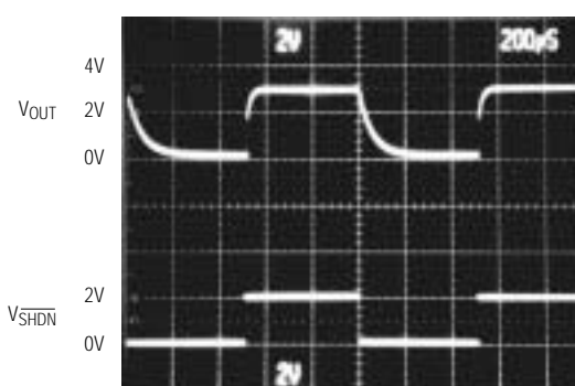
MAX8874 SHUTDOWN
