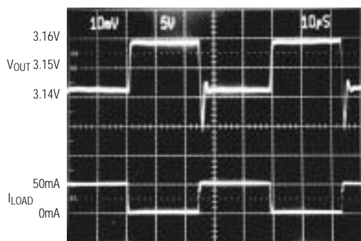
LOAD-TRANSIENT RESPONSE
