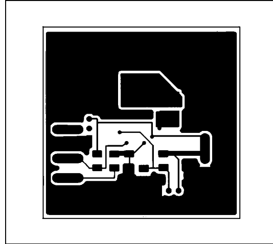
Figure 5. MAX856 EV Kit PC Board Layout—Solder Side
