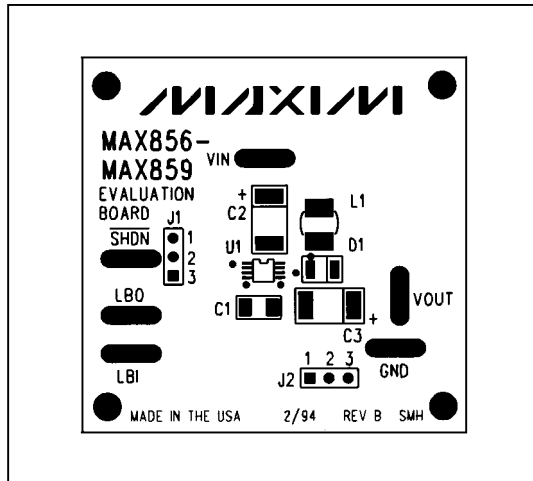
Figure 2. MAX856 EV Kit Component Placement Guide—Component Side
