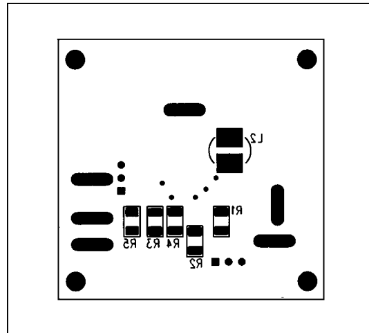
Figure 3. MAX856 EV Kit Component Placement Guide—Solder Side
