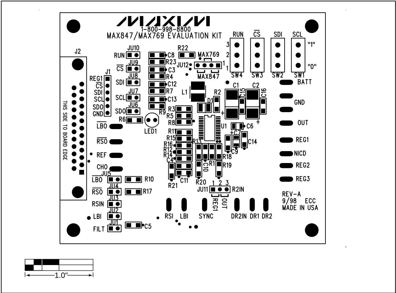
Figure 2. MAX847 EV Kit Component Placement Guide—Component Side
