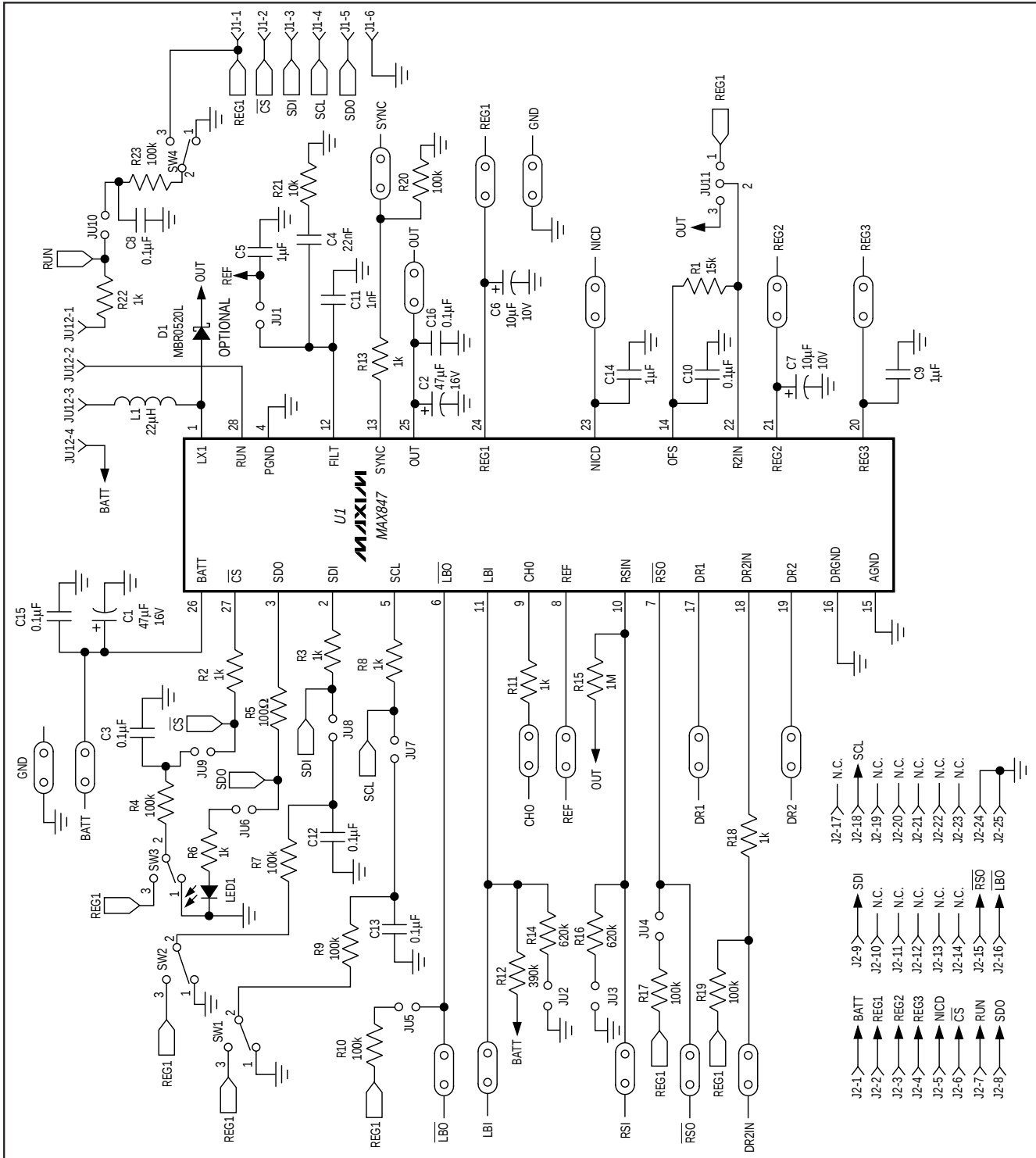
Figure 1. MAX847 EV Kit Schematic
