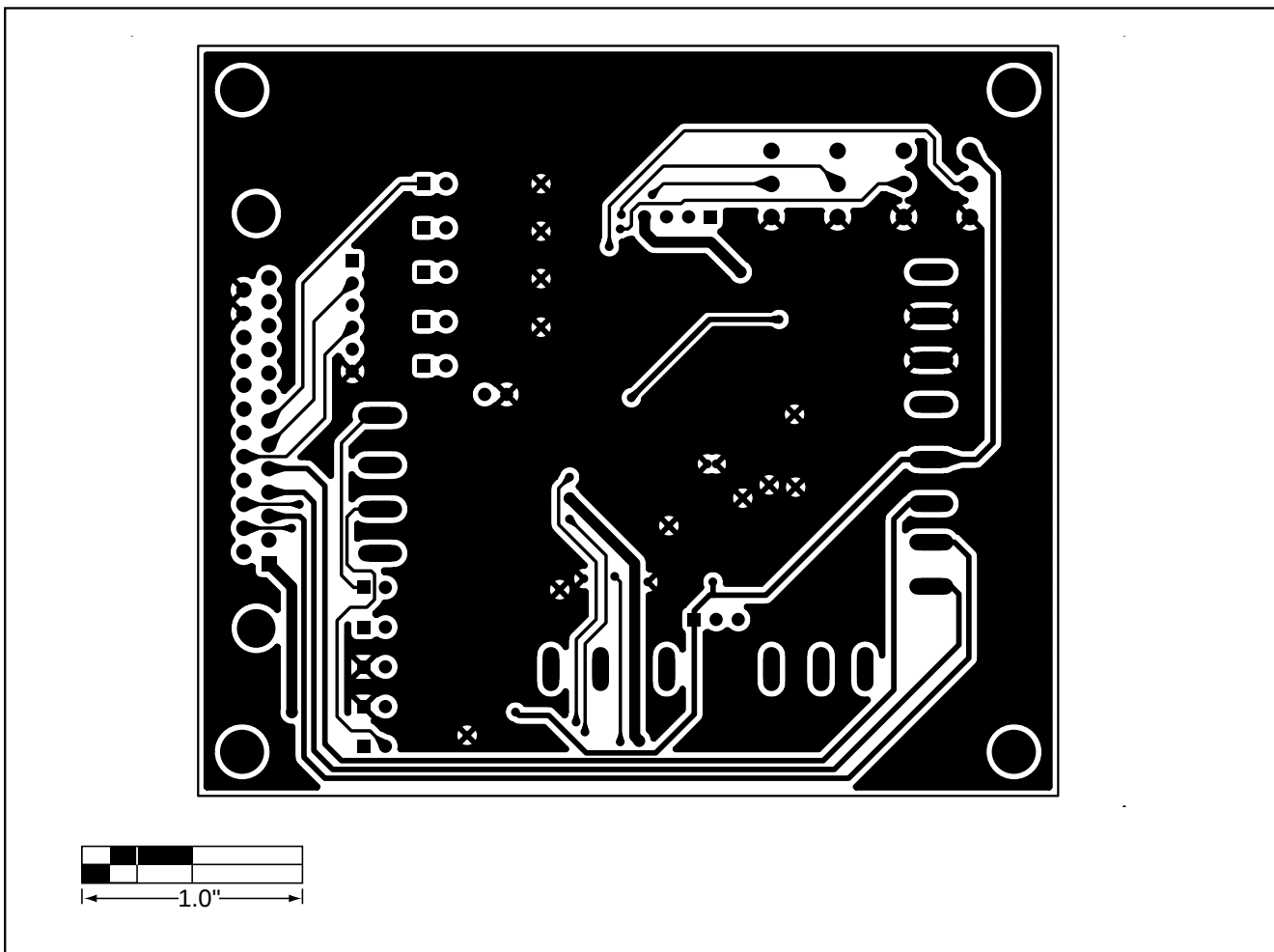
Figure 4. MAX847 EV Kit PC Board Layout—Solder Side
