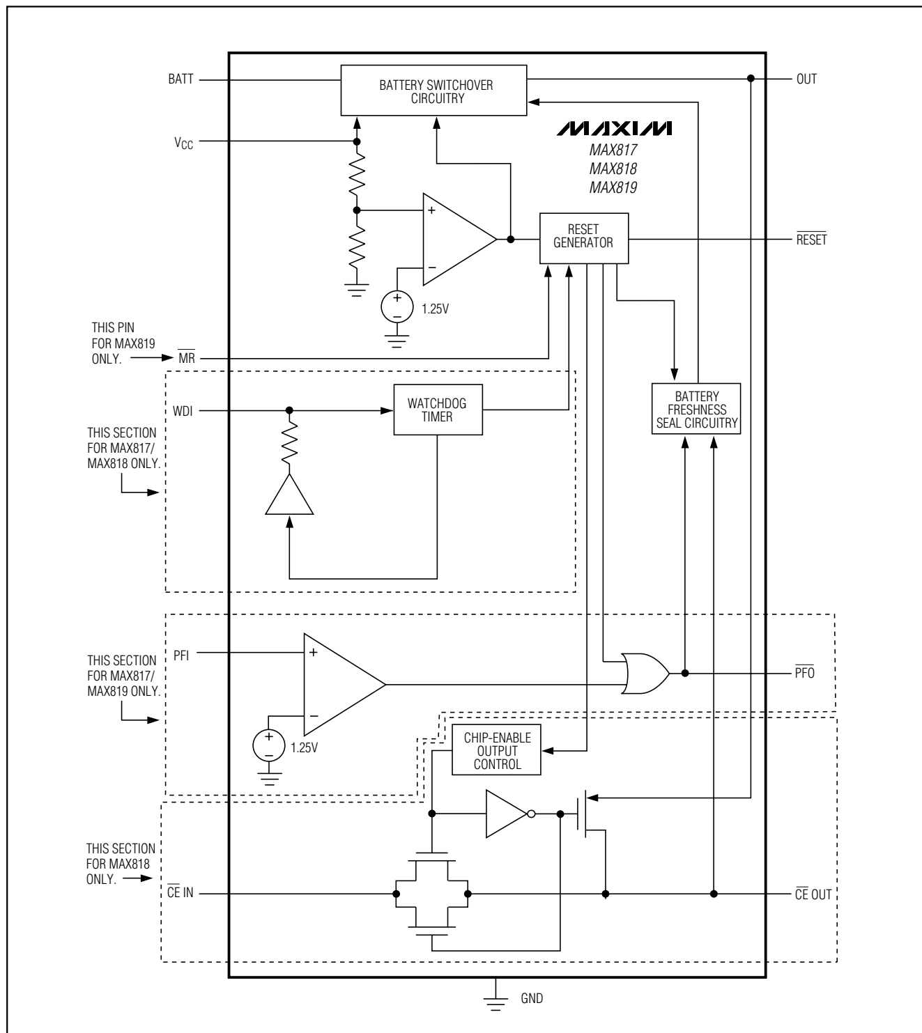
Figure 1. Functional Diagram
