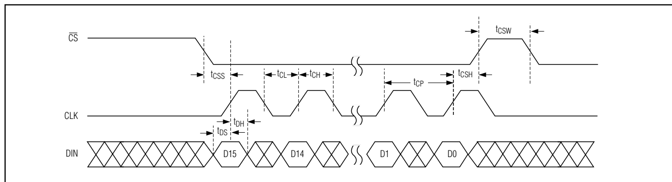
Figure 1. Timing Diagram
