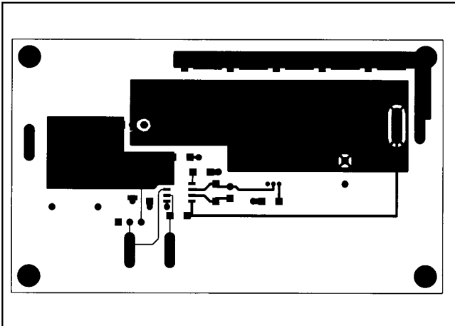
Figure 3. PC Board Layout—Component Side
