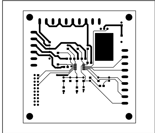
Figure 3. MAX6651 EV Kit PC Board Layout—Component Side
