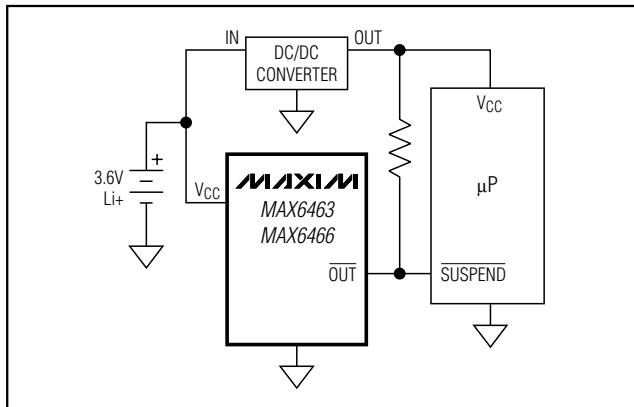
Figure 1. Interfacing to Different Logic Voltage Components
