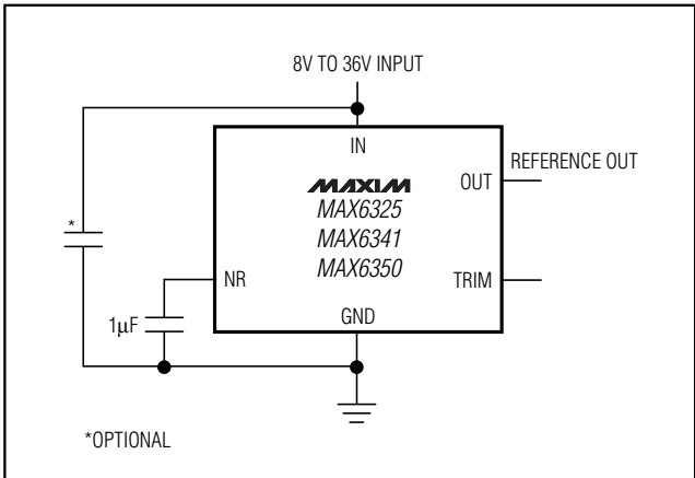
Figure 2. Noise-Reduction Capacitor
