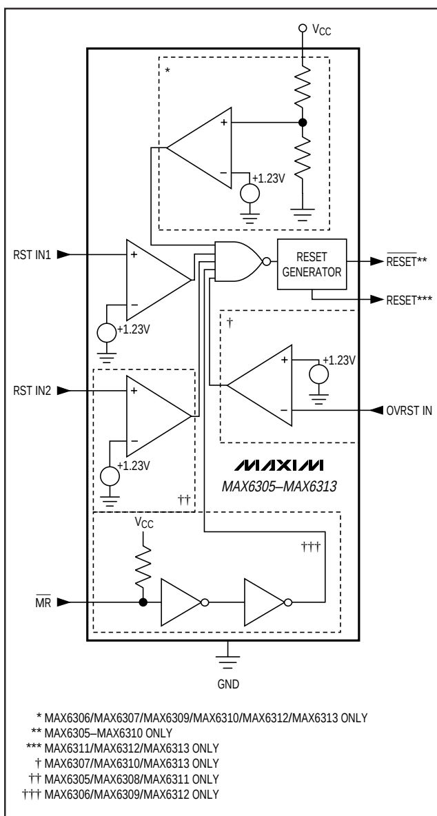
Figure 1. Functional Diagram
