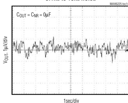
MAX6241 0.1Hz to 10Hz NOISE
