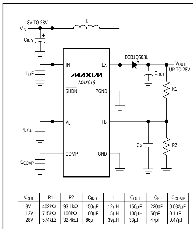
Figure 1. Single-Supply Operation
