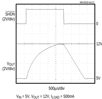
SHUTDOWN RESPONSE
