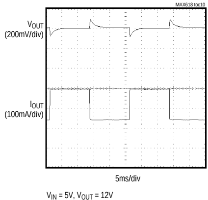
LOAD-TRANSIENT RESPONSE
