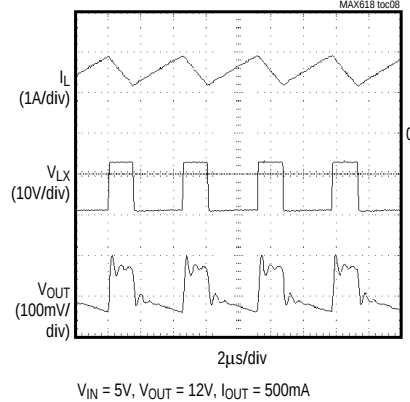
HEAVY-LOAD SWITCHING WAVEFORMS
