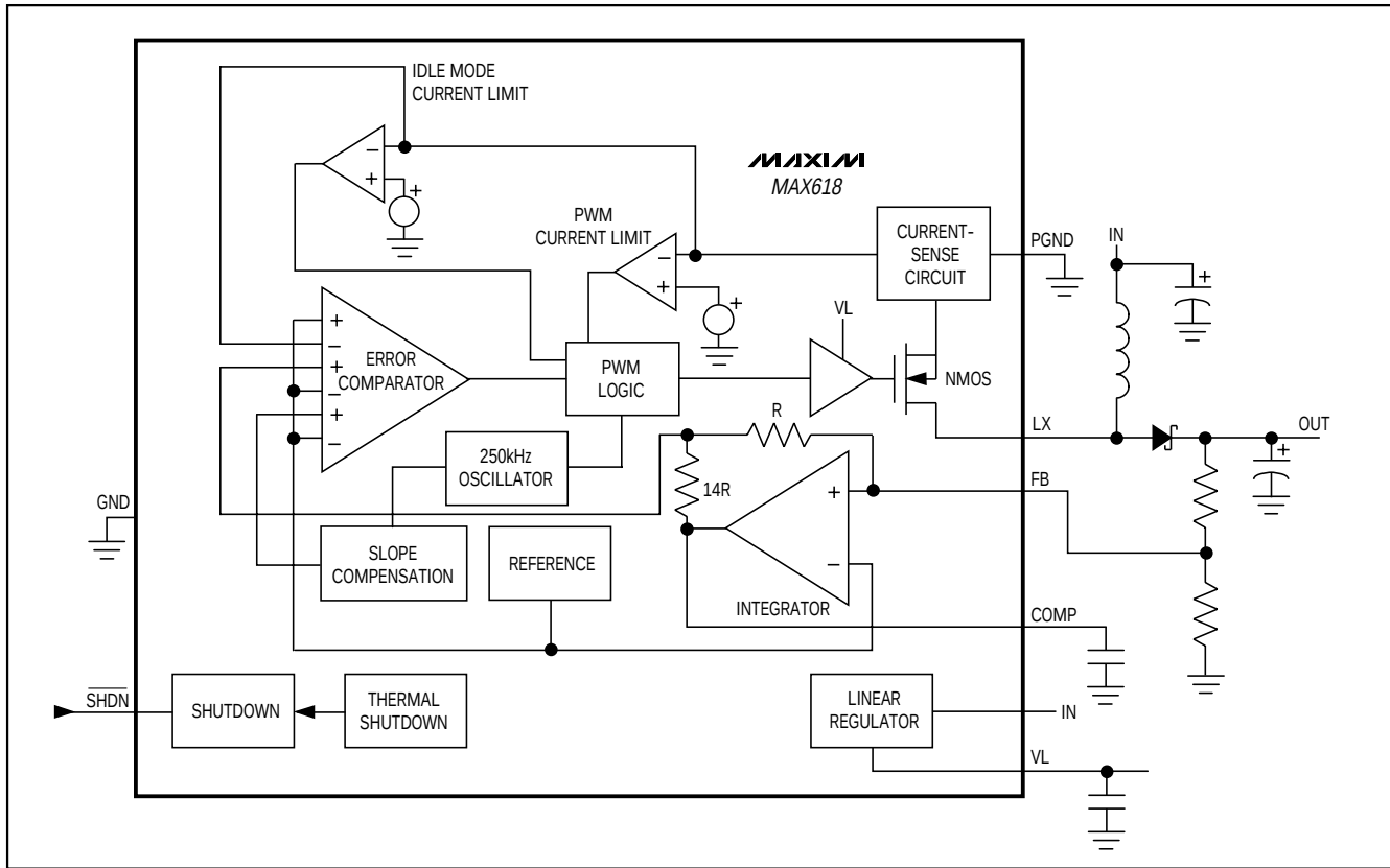
Figure 2. Functional Diagram
