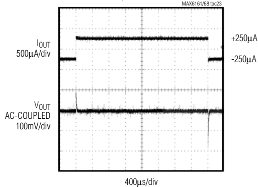
MAX6161 LOAD TRANSIENT ( I_{OUT} = \pm 250\mu A , V_{IN} = 5.0 , C_L = 0 )
