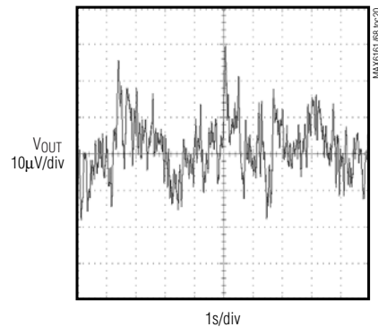
MAX6165 NOISE
