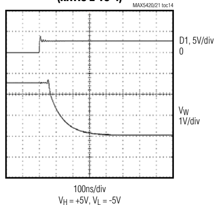
SWITCHING TIME (RATIO 2-T0-4)
