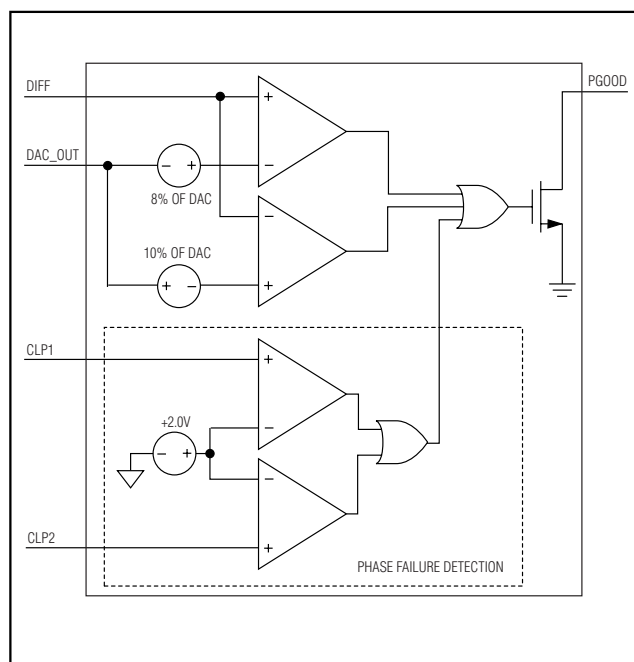
Figure 9. Power-Good Generator
