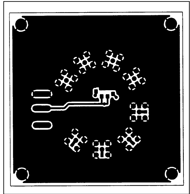
Figure 5. MAX497EV Kit PC Board Layout—Solder Side
