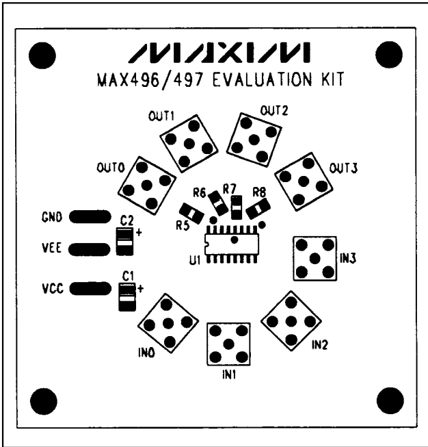
Figure 2. MAX497EV Kit Component Placement Guide—Component Side
