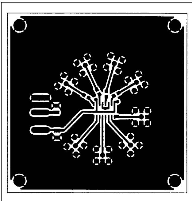
Figure 4. MAX497EV Kit PC Board Layout—Component Side
