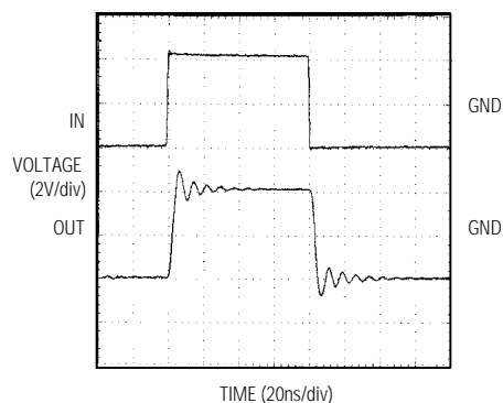
LARGE-SIGNAL PULSE RESPONSE ( A_{vCL} = +1V/V , C_L = 100pF )
