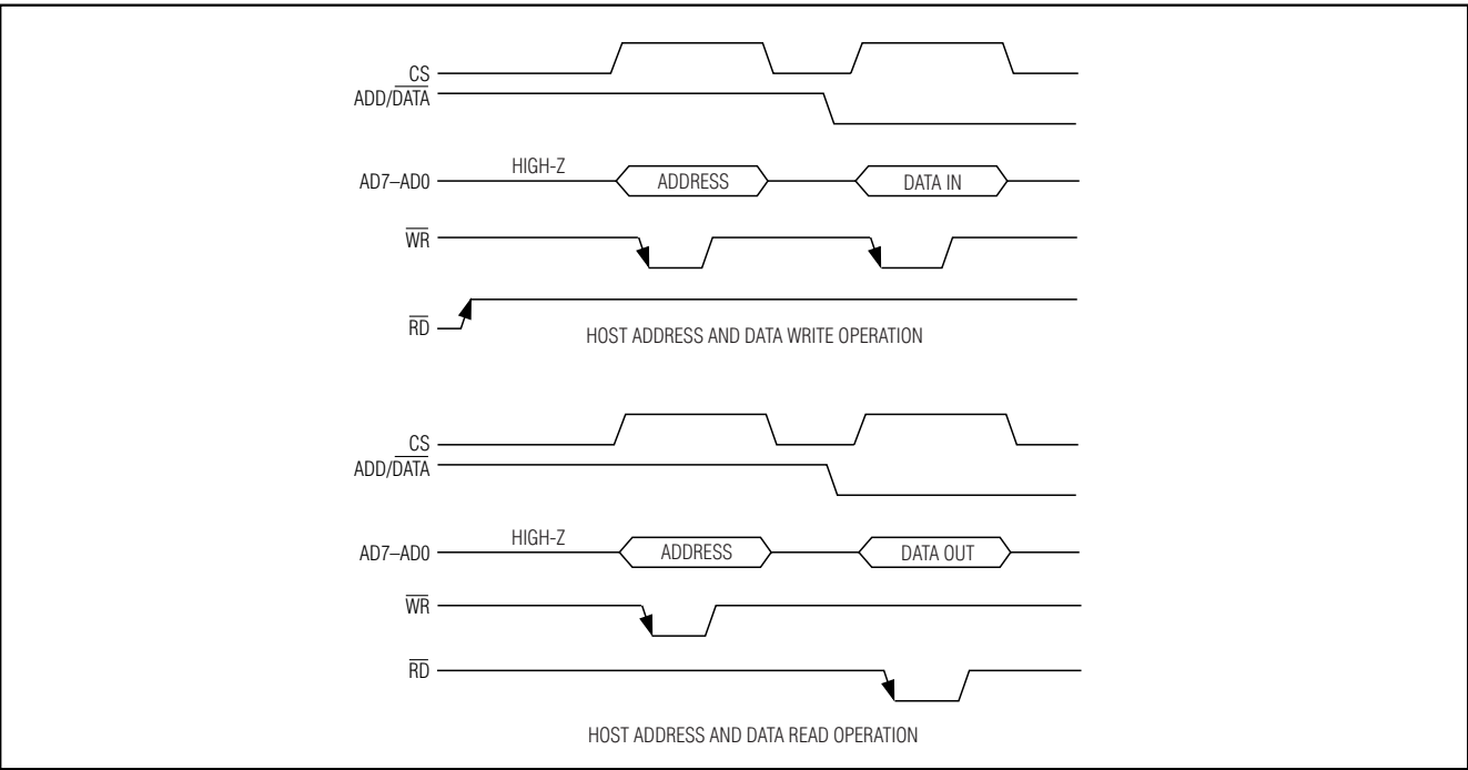
Figure 5. Host Data Write and Read Sequences
