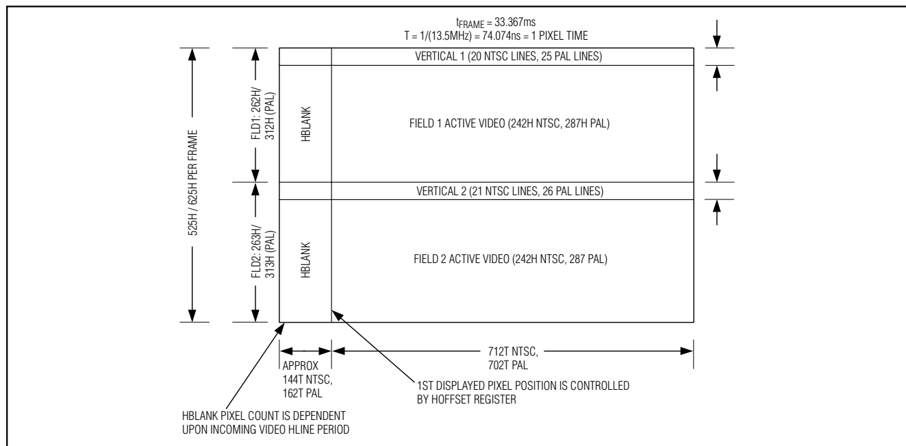
Figure 3. OSD Raster Dimensions
