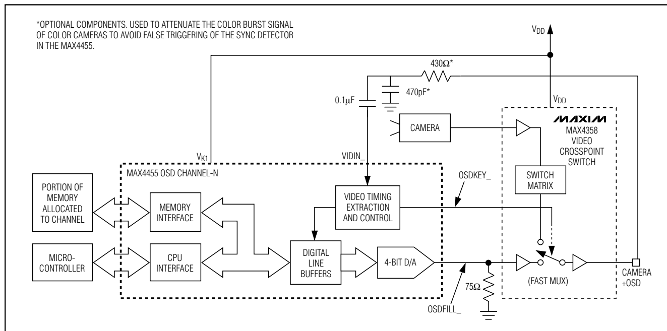
Figure 6. Interfacing MAX4455 with MAX4358 Video Crosspoint Switch
