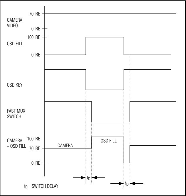
Figure 9. Finite Switch Time Effects
