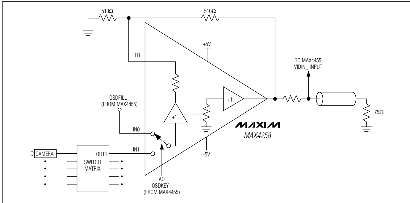
Figure 7. Interfacing MAX4455 with a Fast Mux Switch
