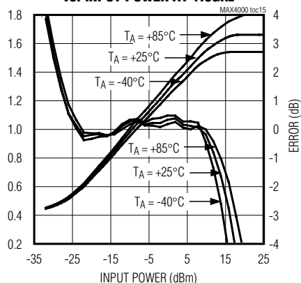
MAX4002 SET AND LOG CONFORMANCE vs. INPUT POWER AT 1.9GHz
