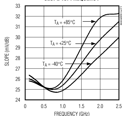
MAX4002 SLOPE vs. FREQUENCY
