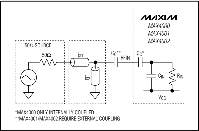
Figure 3b. Narrowband Reactive Matching
