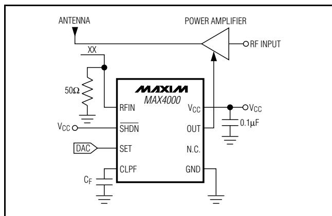
Figure 2. Controller Mode Application Circuit Block
