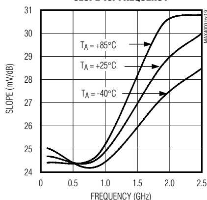
MAX4000 SLOPE vs. FREQUENCY
