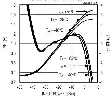
MAX4000 SET AND LOG CONFORMANCE vs. INPUT POWER AT 2.5GHz
