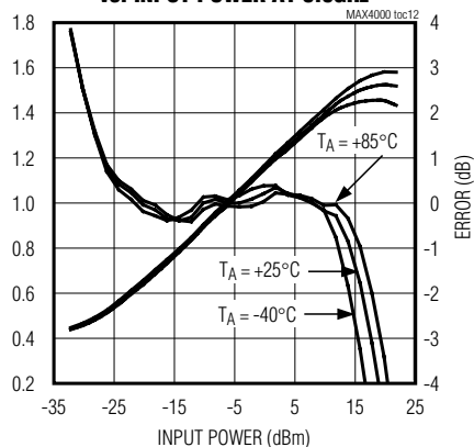
MAX4002 SET AND LOG CONFORMANCE vs. INPUT POWER AT 0.9GHz
