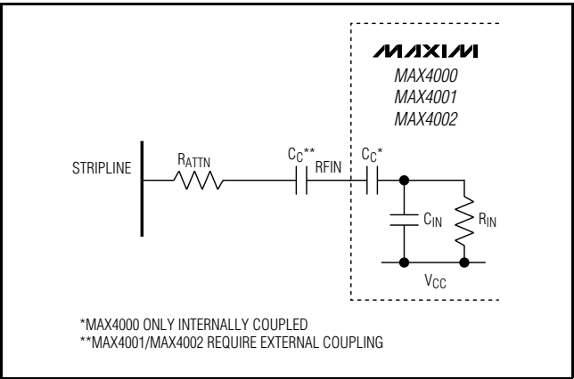
Figure 3c. Series Attenuation Network
