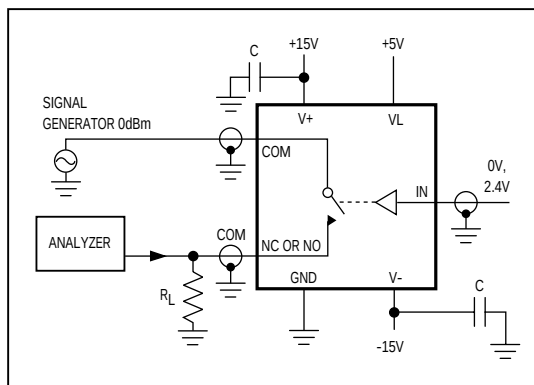
Figure 5. Off-Isolation Test Circuit
