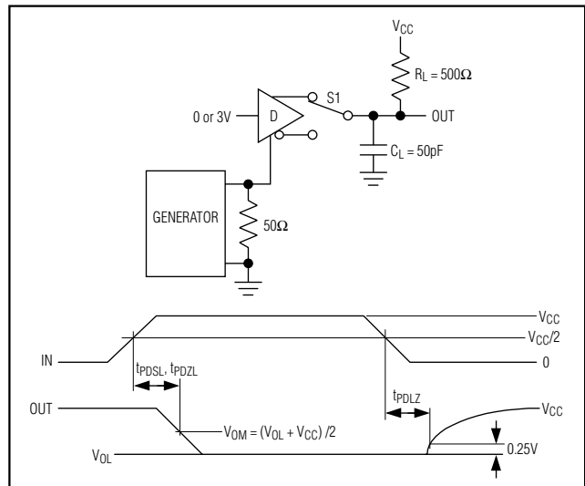
Figure 4. Driver Enable and Disable Times ( t_{PDSL} , t_{PDLZ} , t_{PDLZ} )
