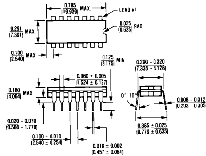
14 Lead CERP (JD) \theta_{JA} = 105^{\circ}\text{C/W} \theta_{JC} = 50^{\circ}\text{C/W}
