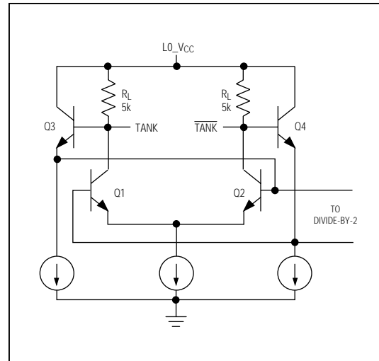
Figure 1. Local-Oscillator Equivalent Circuit
