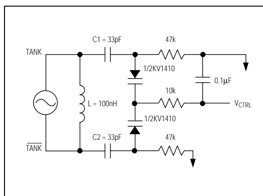
Figure 3. Typical Resonant Tank Circuit
