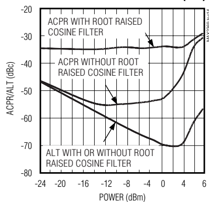
CASCADED ACPR/ALT vs. POWER (RFH)
