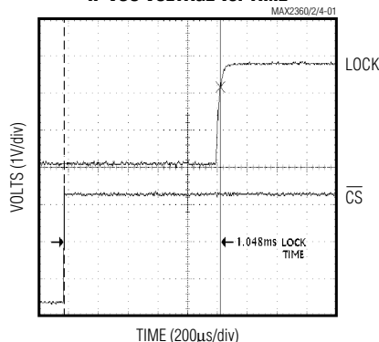
IF VCO VOLTAGE vs. TIME
