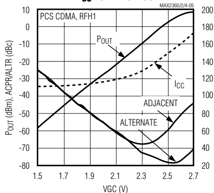
OUTPUT POWER, ACPR, I_{CC} TOTAL vs. VGC
