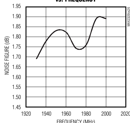
PCS-BAND HGHL LNA NOISE FIGURE vs. FREQUENCY
