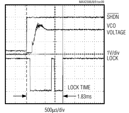
VCO VOLTAGE vs. TIME
