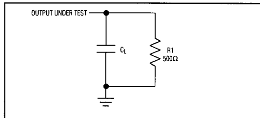
Figure 7. Receiver Enable/Disable Test Circuit 2
