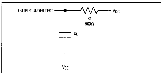
Figure 3. Driver Enable/Disable Test Circuit 1
