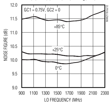
NOISE FIGURE vs. LO FREQUENCY
