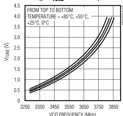
VCO_4: V TUNE vs. VCO FREQUENCY
