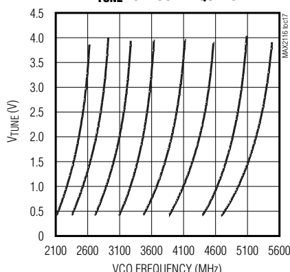
V TUNE vs. VCO FREQUENCY
