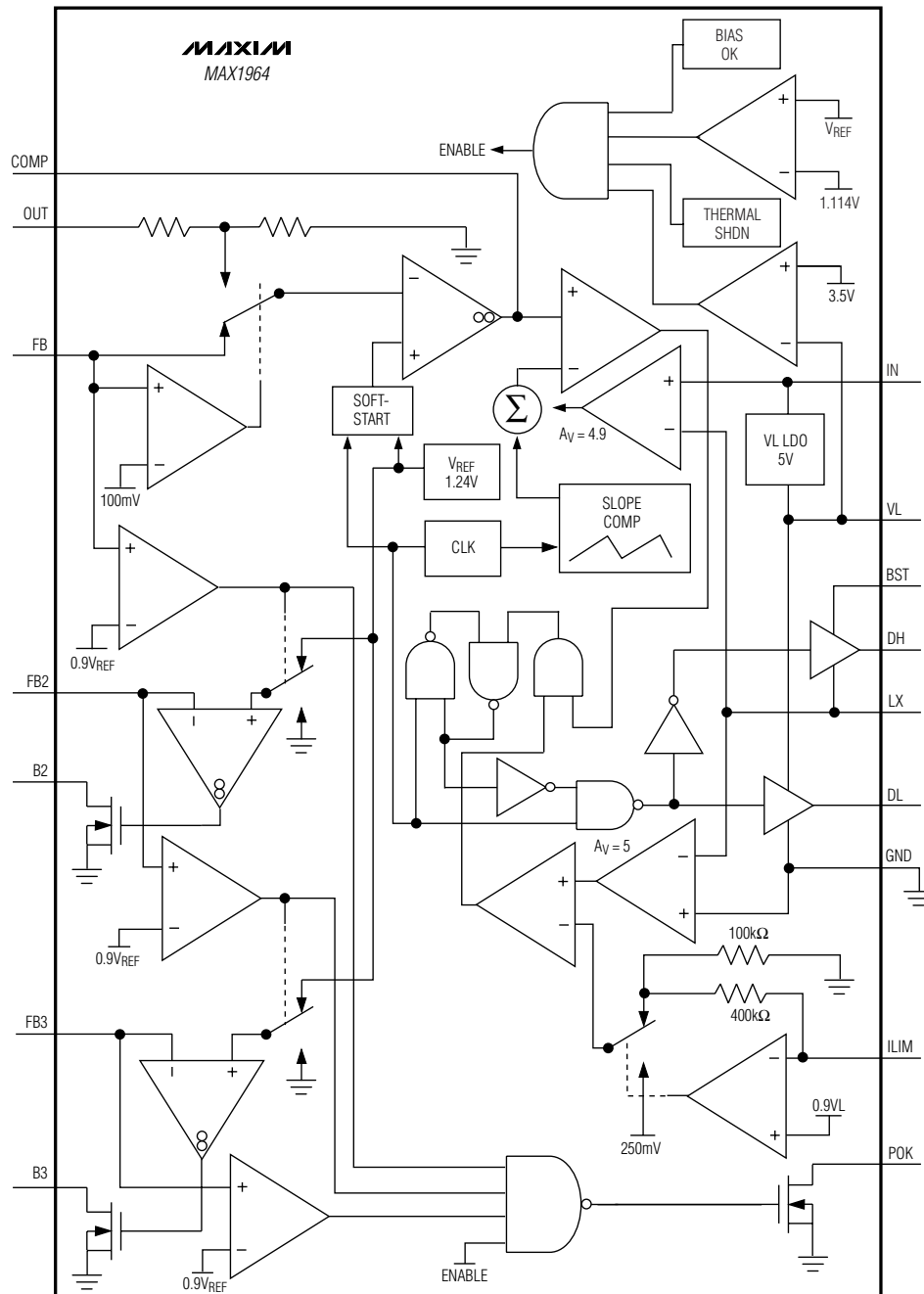
Figure 2a. MAX1964 Functional Diagram
