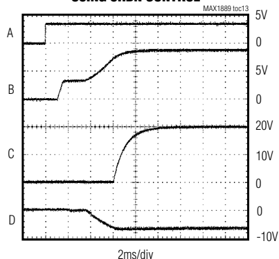
POWER-UP SEQUENCE USING \overline{SHDN} CONTROL
