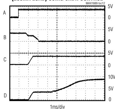
STEP-UP REGULATOR SOFT-START (200mA LOAD) USING \overline{SHDN} CONTROL
