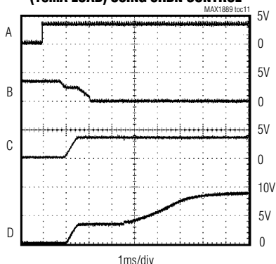
STEP-UP REGULATOR SOFT-START (10mA LOAD) USING \overline{SHDN} CONTROL
