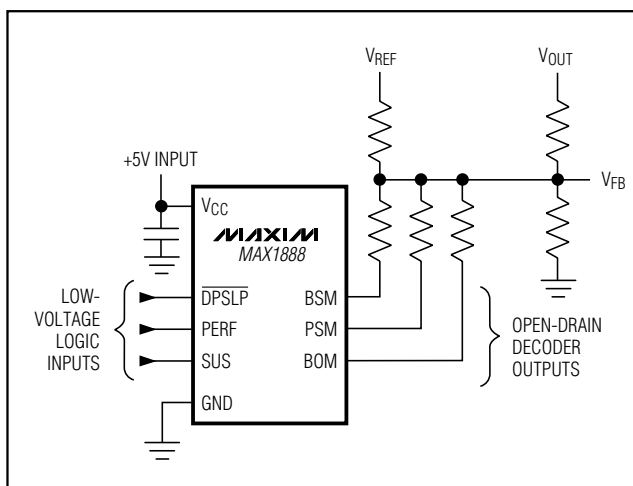
Figure 4. Inserting the MAX1888 into the Feedback Path of Any Regulator to Shift Output Voltage
