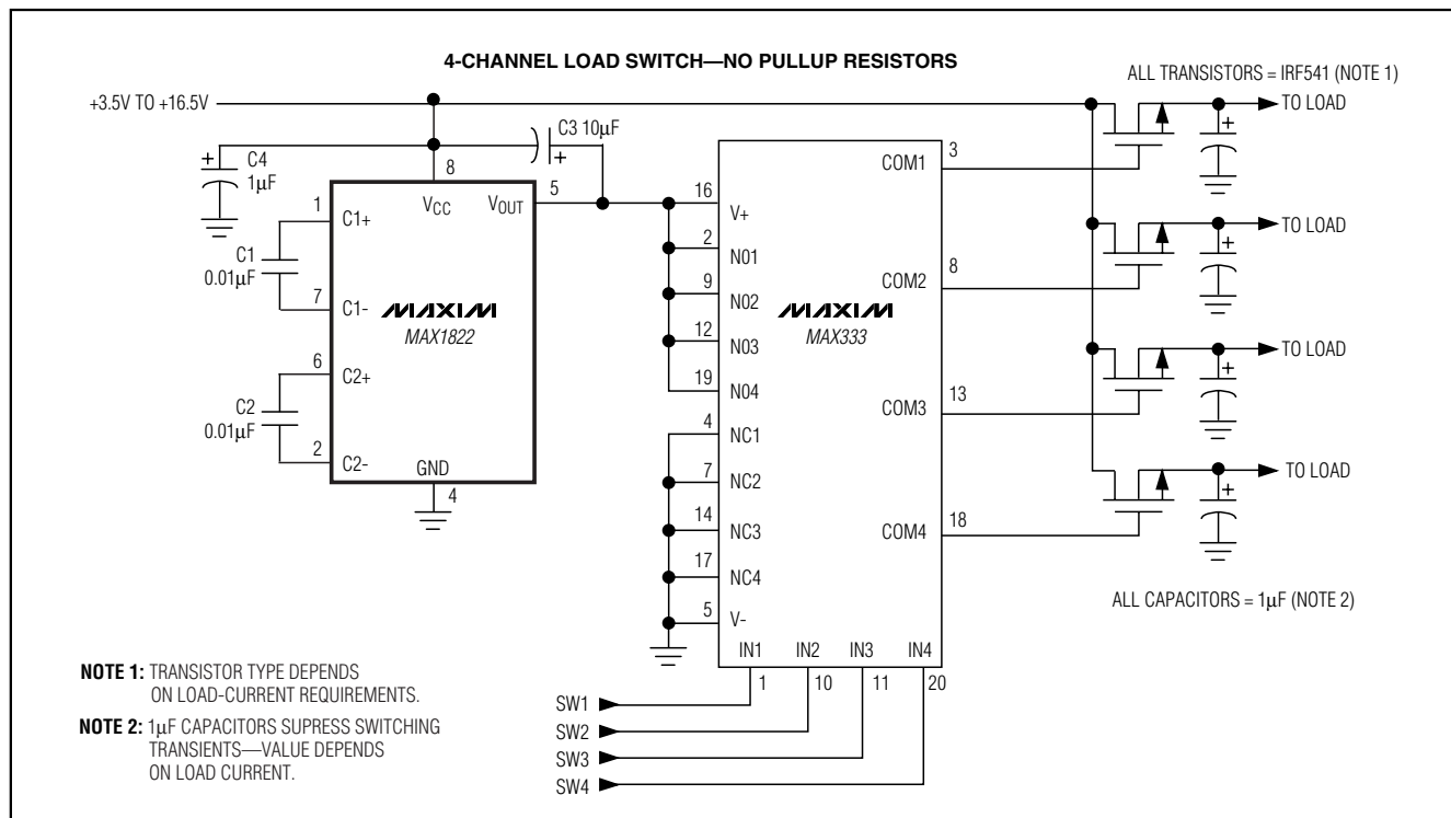
Figure 5. MAX1822 Powering a MAX333 Quad Analog Switch, Realizing a 4-Channel Load Switch with No Pullup Resistors
