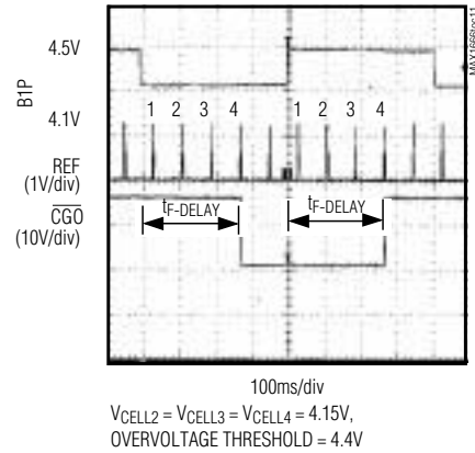
CELL MISMATCH FAULT
