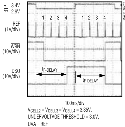
UNDERVOLTAGE FAULT
