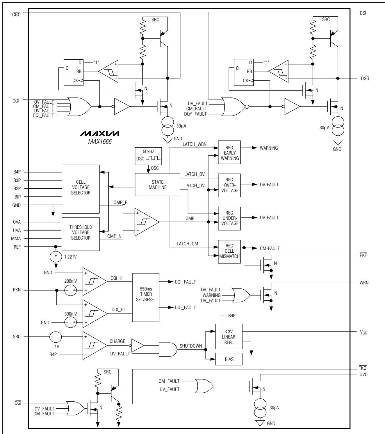
Figure 1. Functional Diagram
