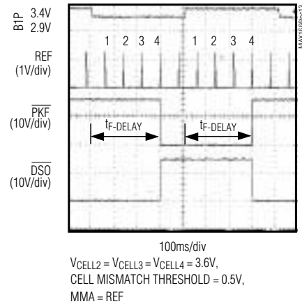
CELL MISMATCH FAULT
