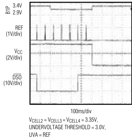
UNDERVOLTAGE FAULT WITHOUT CHARGE SOURCE ( V_{SRC} < V_{B4P} + 1\text{V} )
