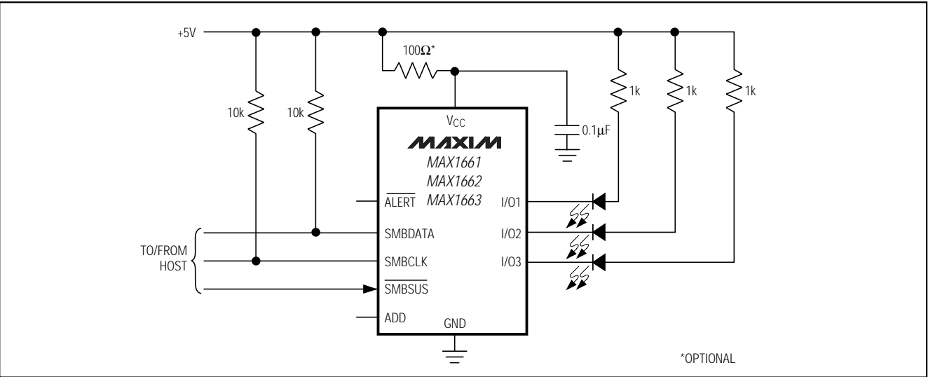
Figure 8. LED Drivers
