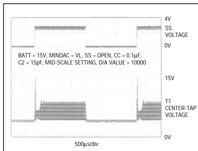
Figure 14. Chopped Waveforms
