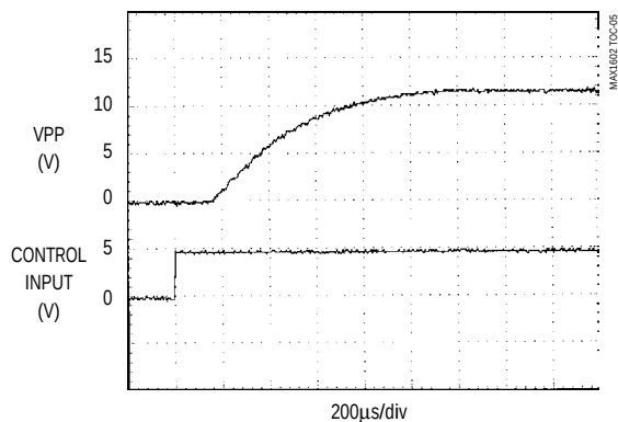
VPP SWITCHING (RISE)
