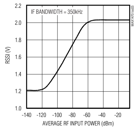
RSSI vs. AVERAGE RF INPUT POWER
