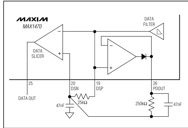
Figure 3. Using PDOUT for Faster Startup
