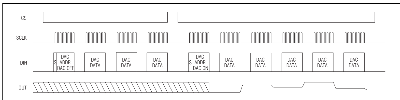
Figure 7. DAC Continuous Conversion Mode Timing Diagram
