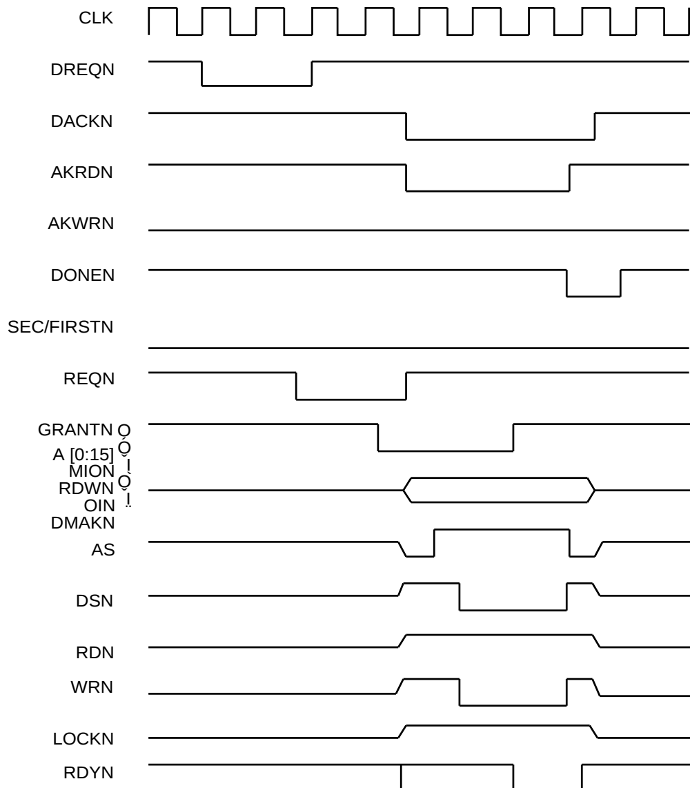
Figure 7: Single Cycle Without Handshake, Memory Write
