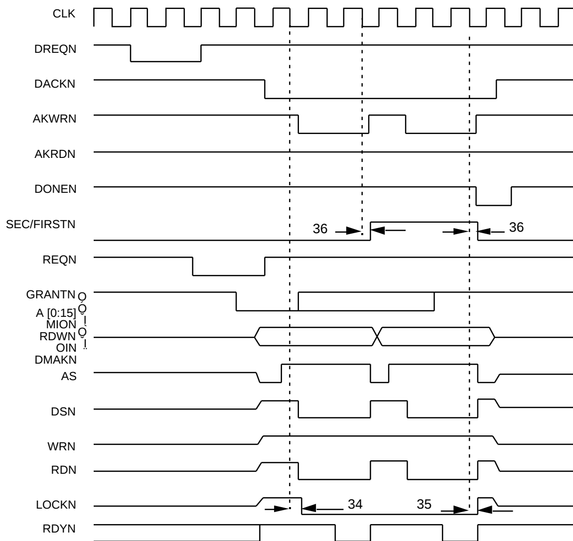
Figure 8: Double Mode, Memory Read
