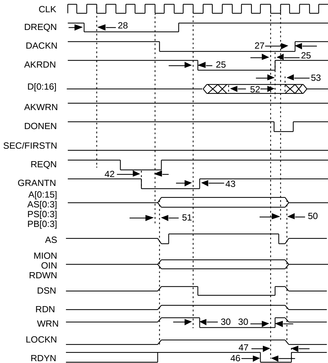
Figure 5: Single Cycle With Handshake, Memory Write
