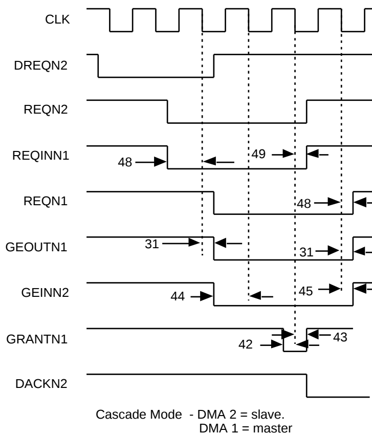
Figure 13: Cascade Mode
