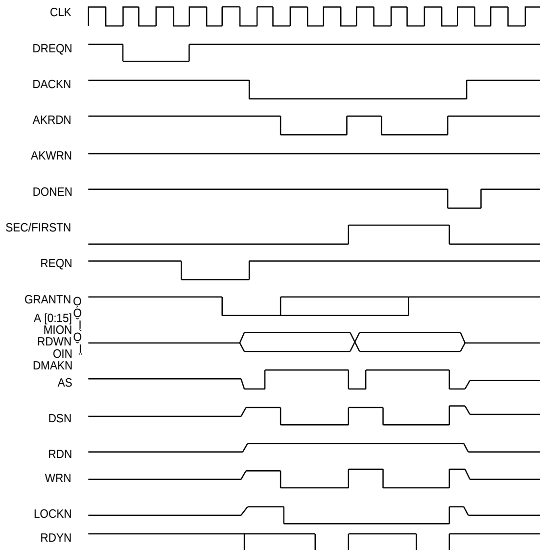
Figure 9: Double Mode, Memory Write
