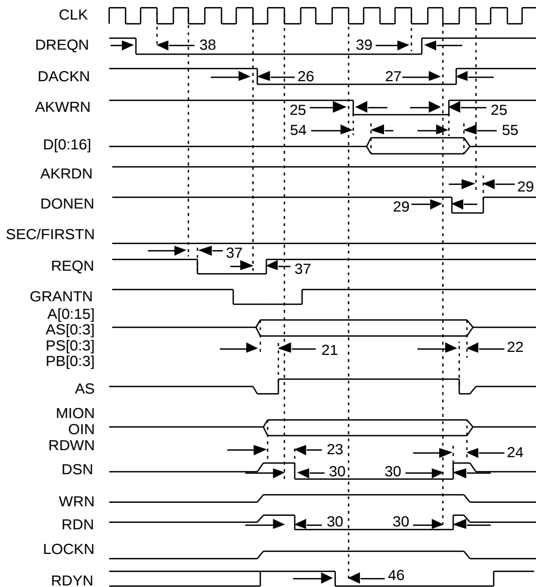
Figure 4: Single Cycle With Handshake, Memory Read
