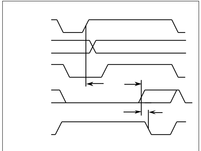
Figure 16: MMU and BPU Timings
