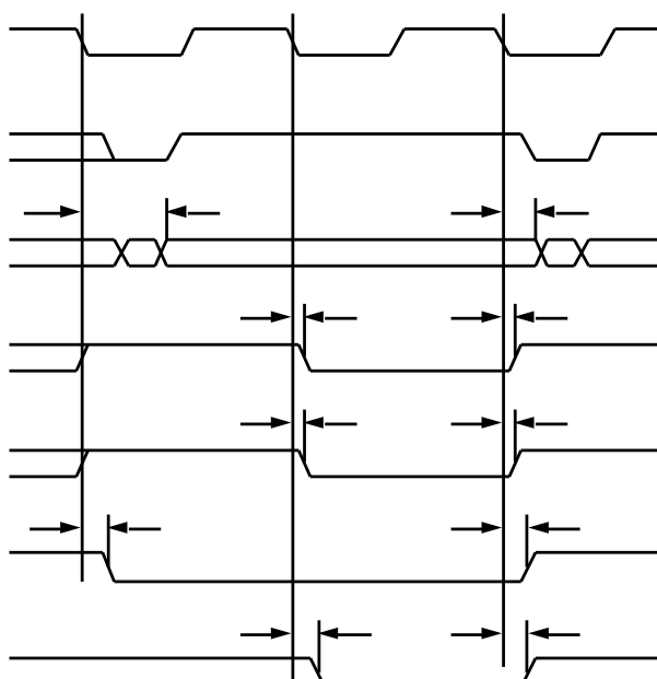
Figure 28: Discrete Timings
