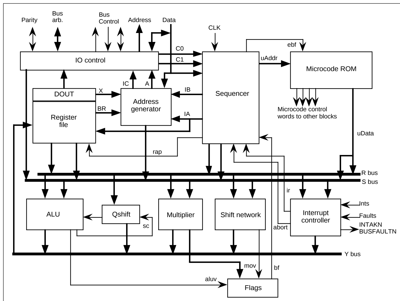
Figure 1: Architecture
