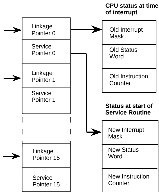
Figure 11: Interrupt Vectoring
