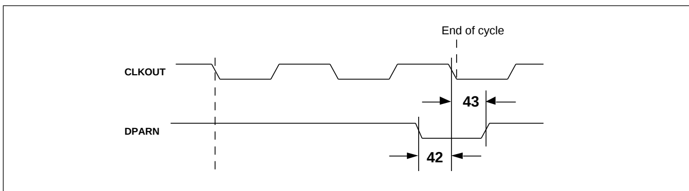
Figure 31: DPARN Timing
