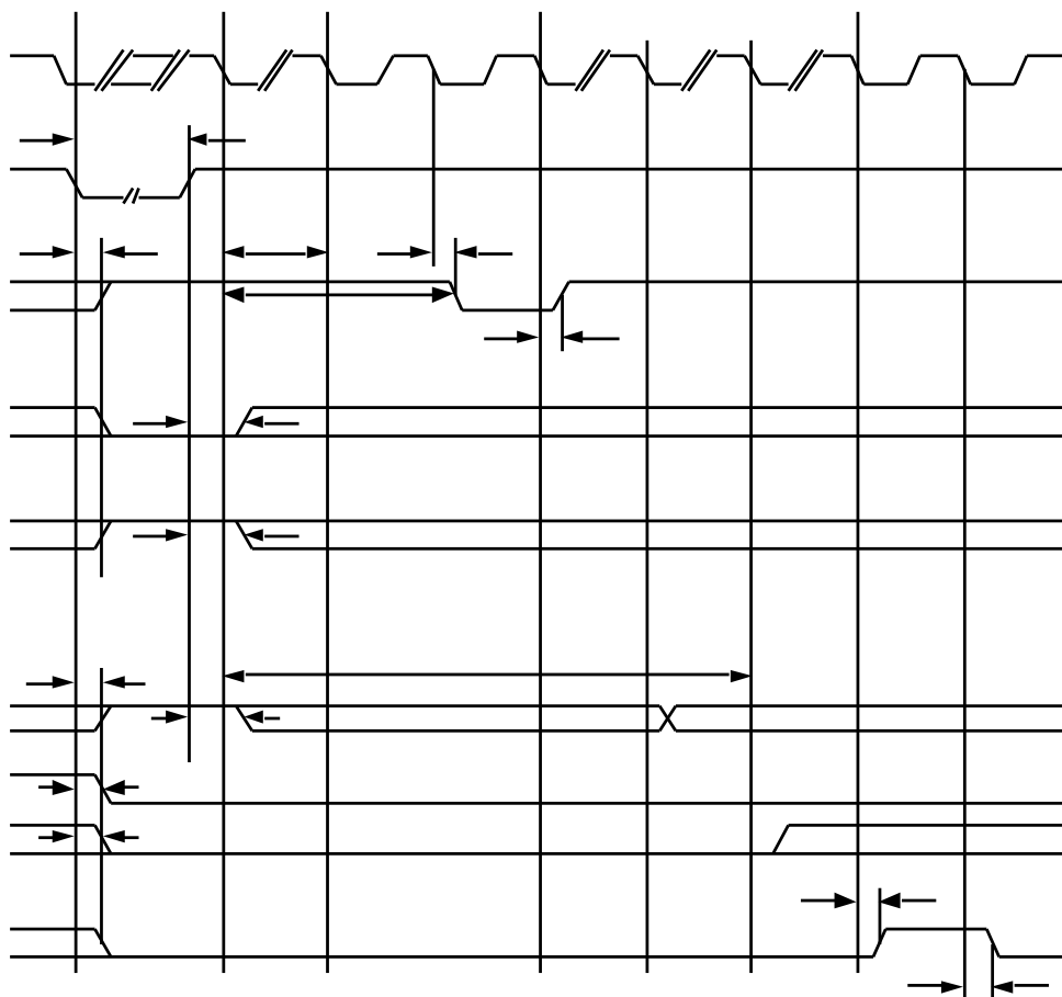
Figure 25: Reset Timing
