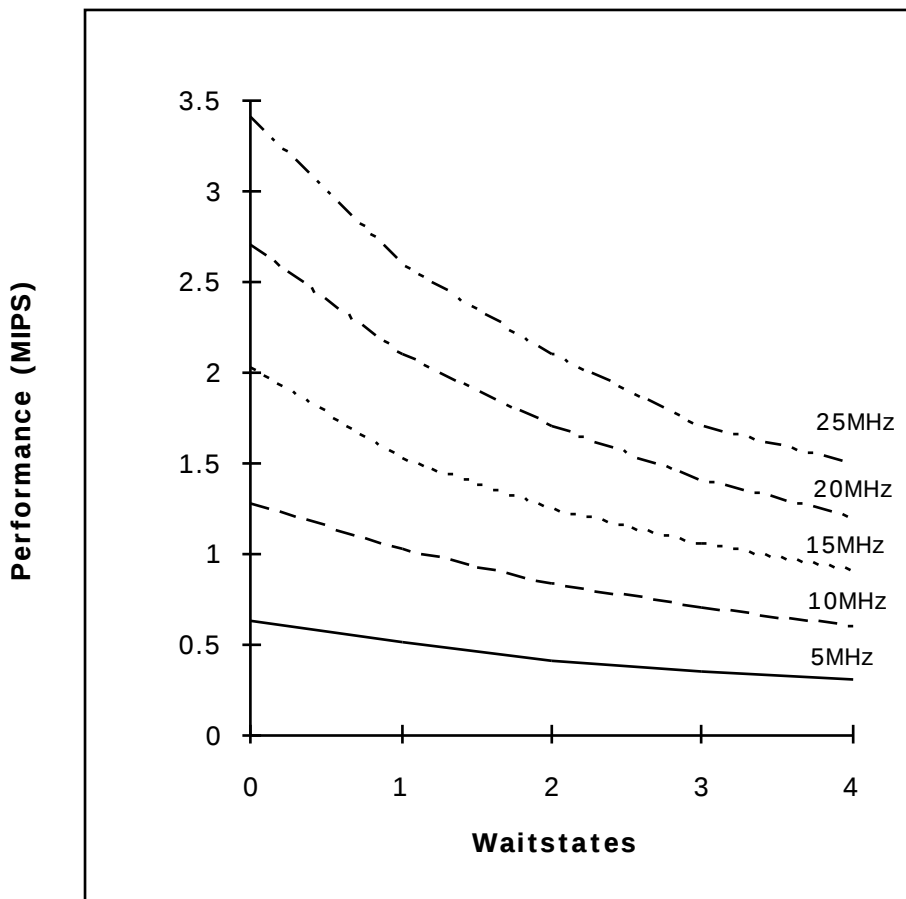
Figure 19: Throughput (MIPS) with Waitstates
