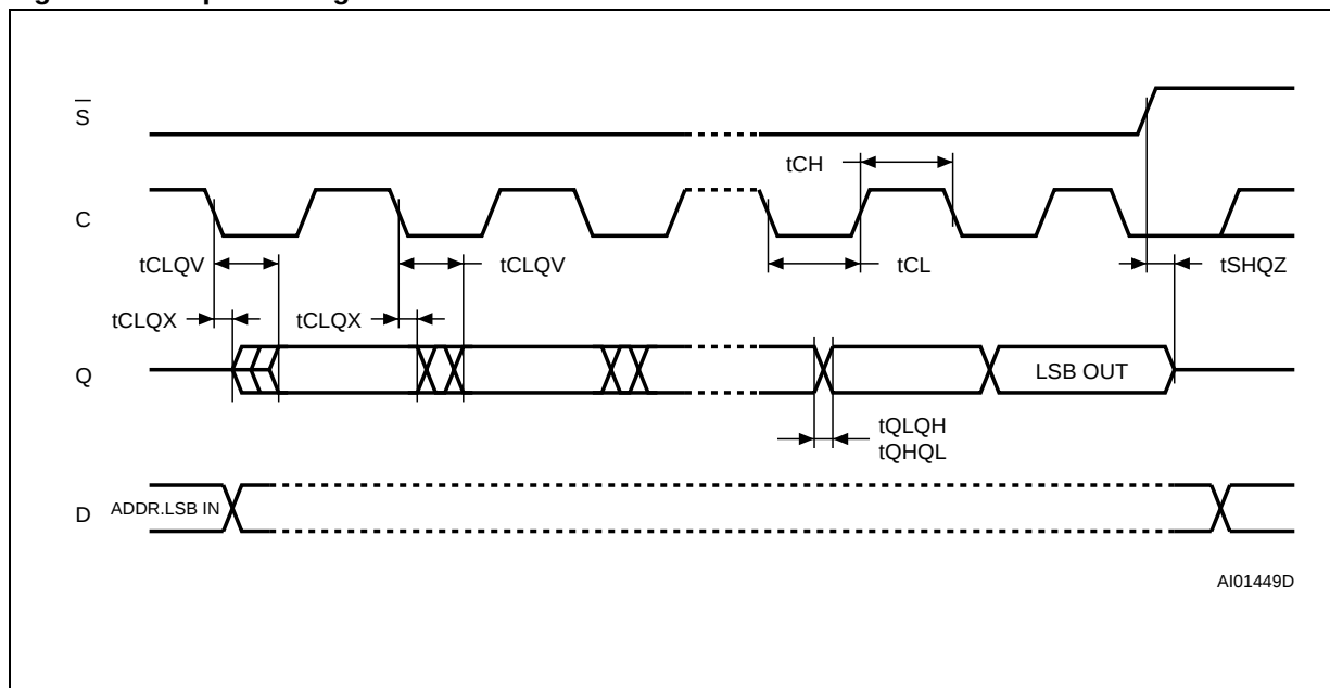
Figure 19. Output Timing
