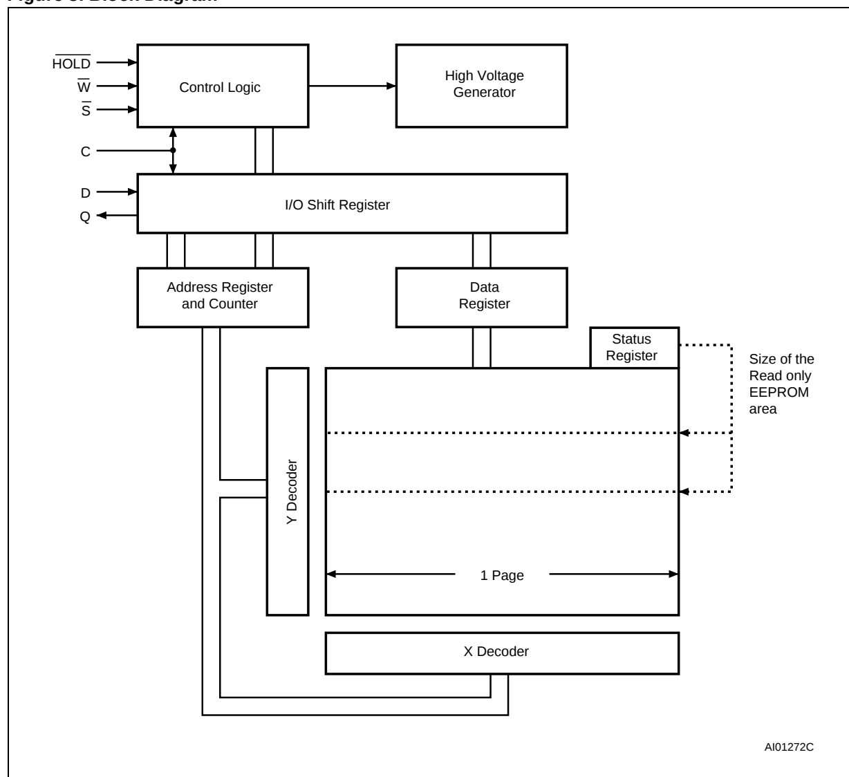
Figure 8. Block Diagram
