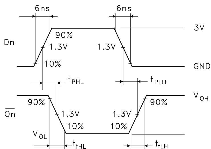
WAVEFORM 3 : PROPAGATION DELAY TIMES ( f=1\text{MHz} ; 50% duty cycle)
