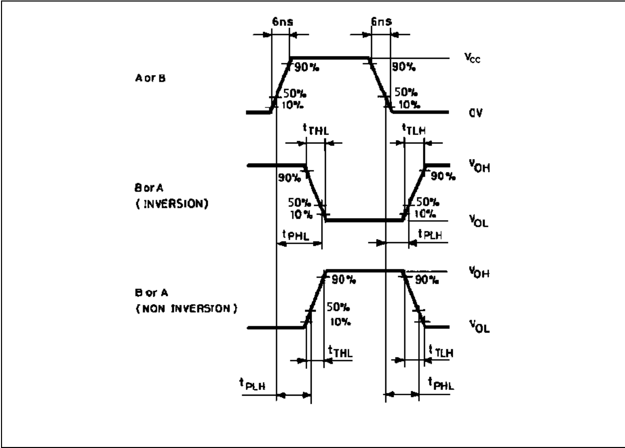
WAVEFORM 1 : PROPAGATION DELAY TIME (f=1MHz; 50% duty cycle)
