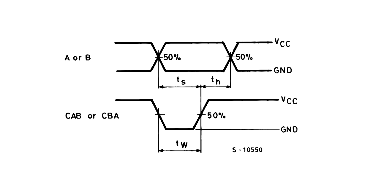
WAVEFORM 3 : MINIMUM PULSE WIDTH, SETUP AND HOLD TIME ( f=1\text{MHz} ; 50% duty cycle)
