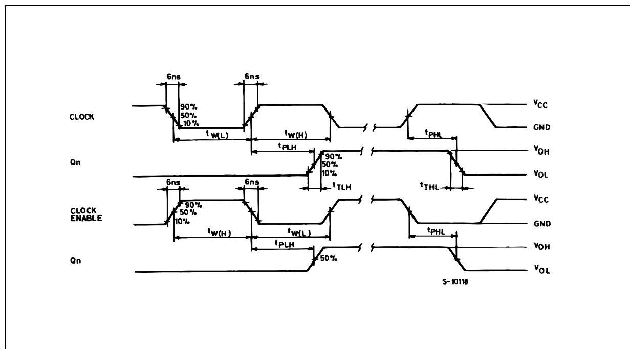
WAVEFORM 2 : PROPAGATION DELAY, MINIMUM PULSE WIDTH AND REMOVAL TIMES (CLOCK AND CE) ( f=1\text{MHz} ; 50% duty cycle)
