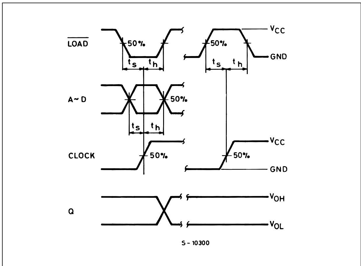
WAVEFORM 3 : MINIMUM SETUP AND HOLD TIME ( f=1\text{MHz} ; 50% duty cycle)
